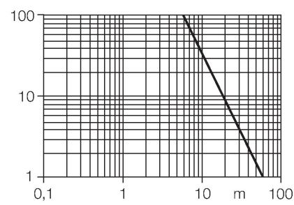
Caracteristica "Excess gain"
